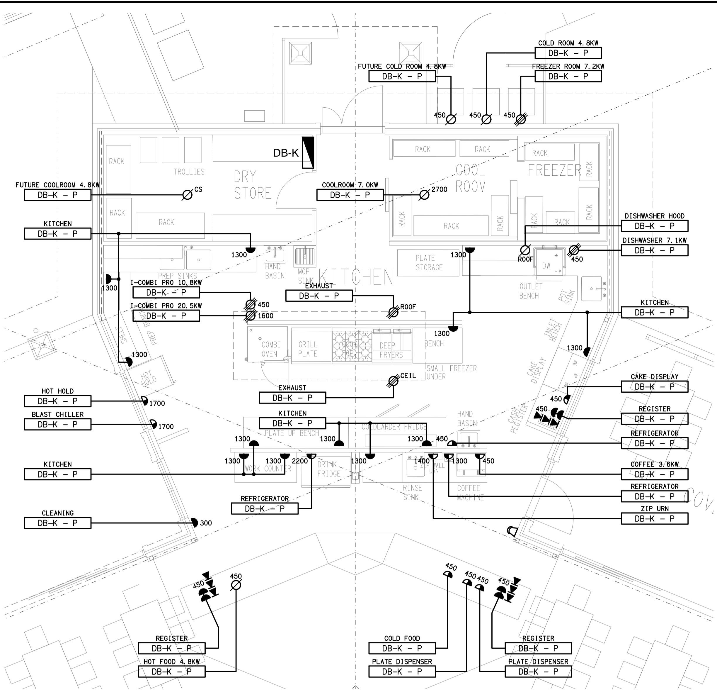
DETAIL A KITCHEN FLOOR PLAN SCALE 1: 50
